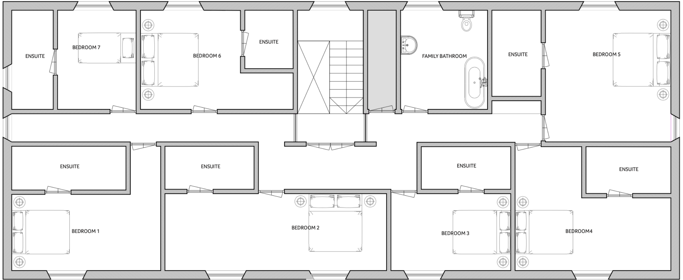
FIRST FLOOR
